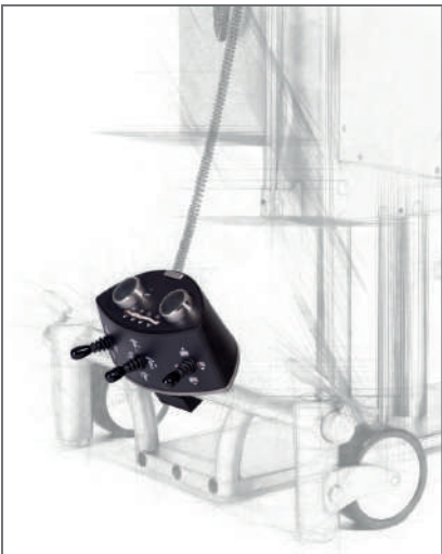
FOOT CONTROL, TYPE IV FIXED ON UNDERCARRIAGE
